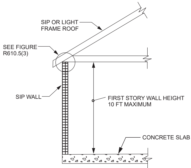
FIGURE R610.5(1) MAXIMUM ALLOWABLE HEIGHT OF SIP WALLS
