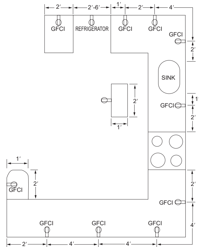
FIGURE E3901.4 COUNTERTOP RECEPTACLES
