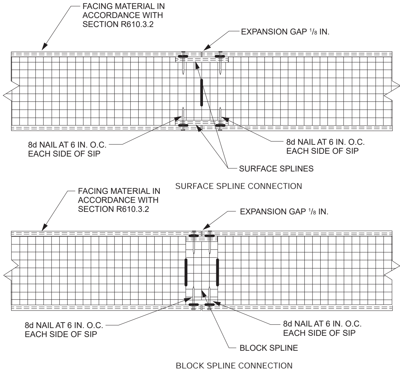
FIGURE R610.8 TYPICAL SIP CONNECTION DETAILS FOR VERTICAL IN-PLANE JOINTS
