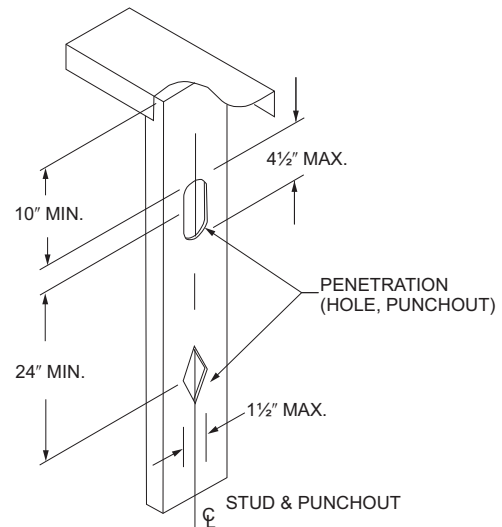
FIGURE R603.2.6.1 WALL STUD WEB HOLES
