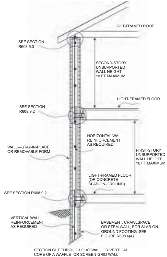
FIGURE R608.6(3) ABOVE-GRADE CONCRETE WALL CONSTRUCTION TWO-STOREY
