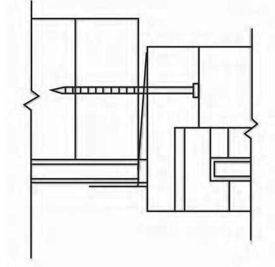
FIGURE R609.7.2(6) THROUGH THE FLANGE
