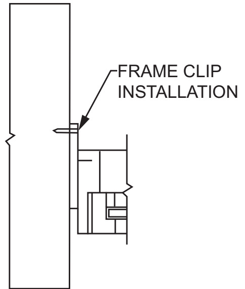
FIGURE R609.7.2(2) FRAME CLIP
