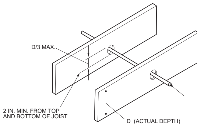
FIGURE R502.8 CUTTING, NOTCHING AND DRILLING
